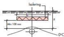
Figur 24. Horisontell isolering.
